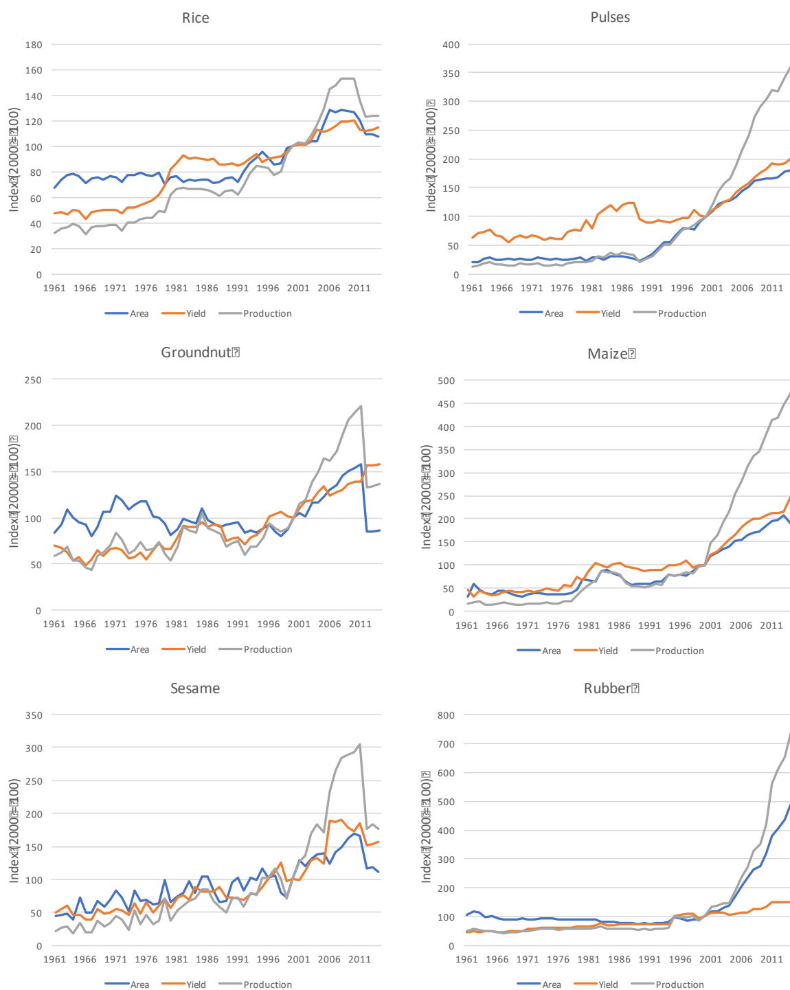
Figure 3.6: Change in area, yield and production for main crops in Myanmar 1961-2014
