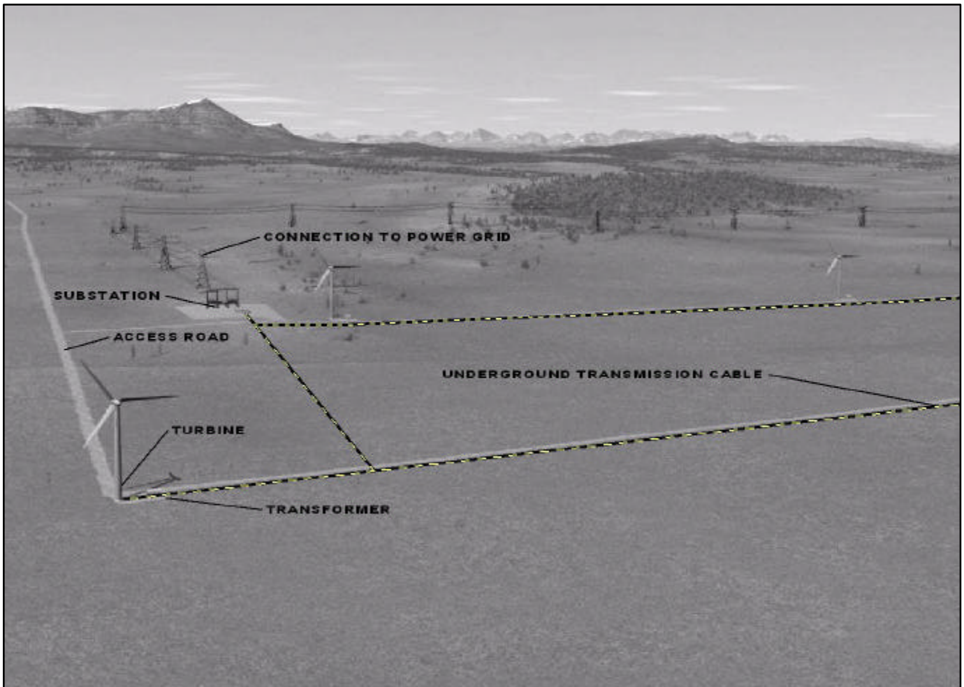
Figure A-2. Typical Components of an Onshore Wind Farm
